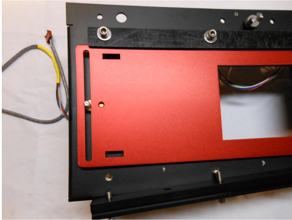
Vat Table in place, note motor arm with nylon spacer in table slot. Front track ready to mount.
