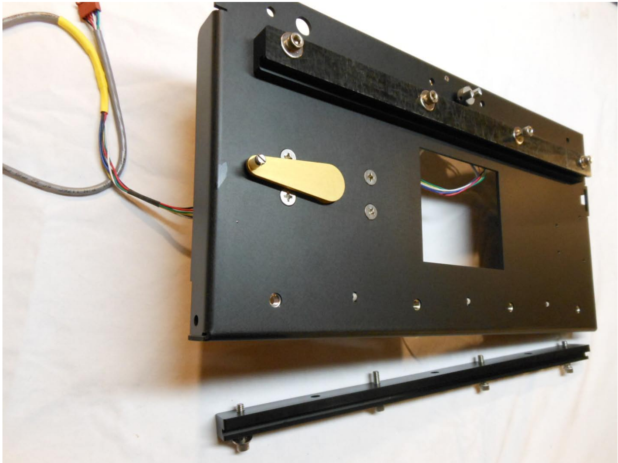
Back track in place, screws only hand tightened
