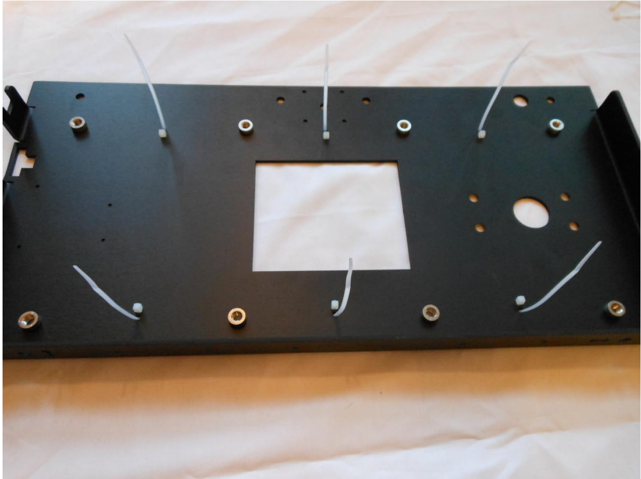
Bottom View - All six in place, note how they are positioned with long ends towards the outside edge to make it easier to tighten them later.
