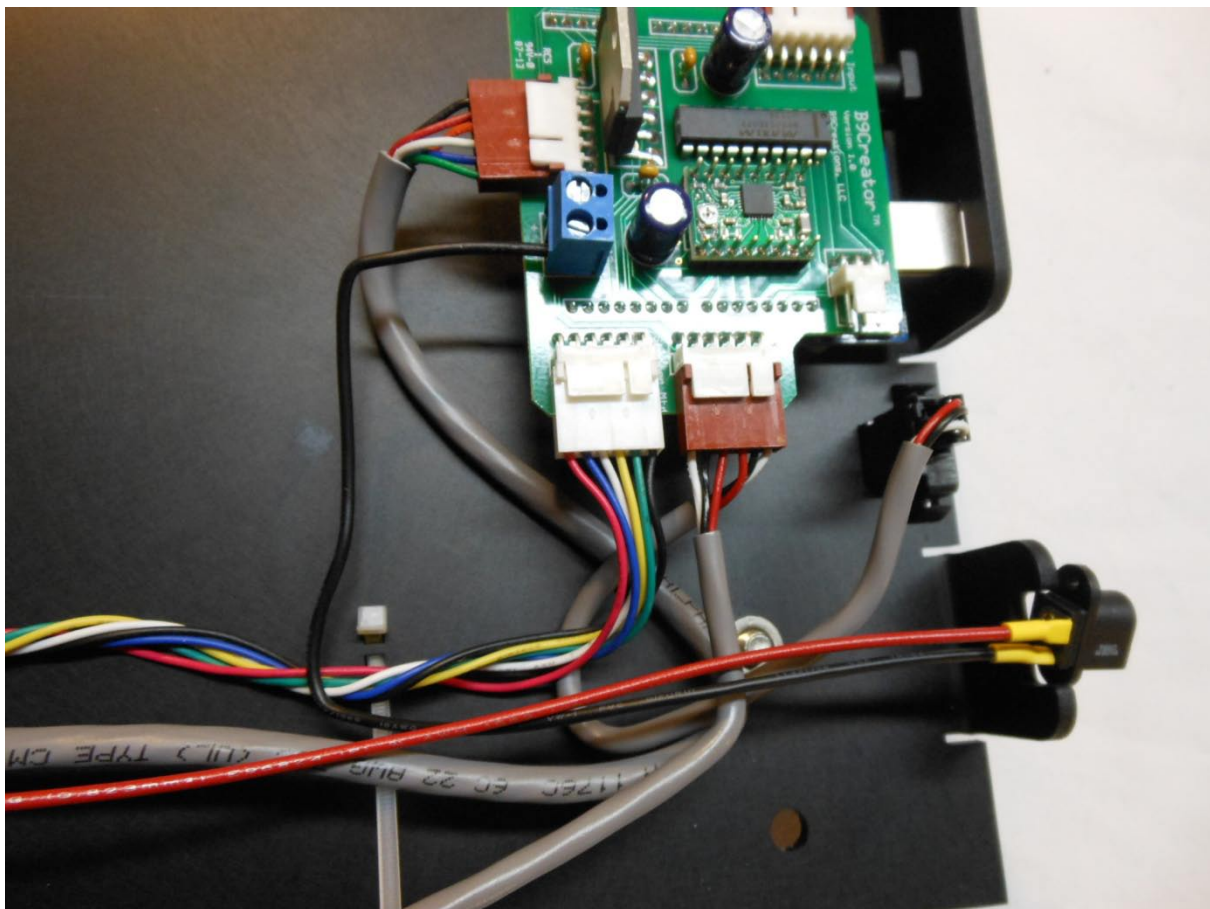
Power input in place with black wire connected to negative (-) Shield terminal
