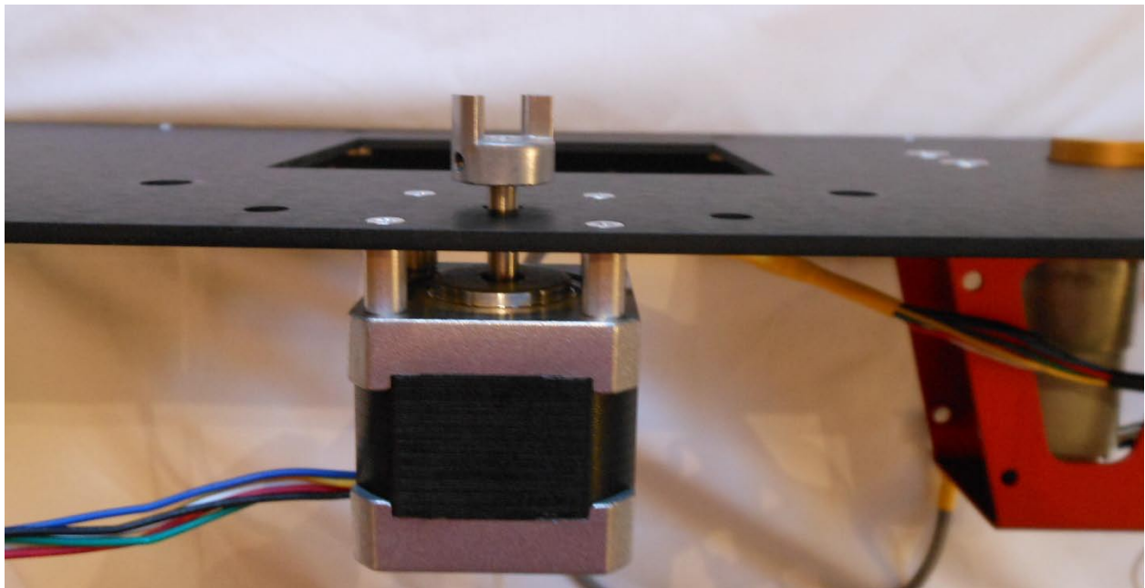
Z Axis Stepper Moto Installed
