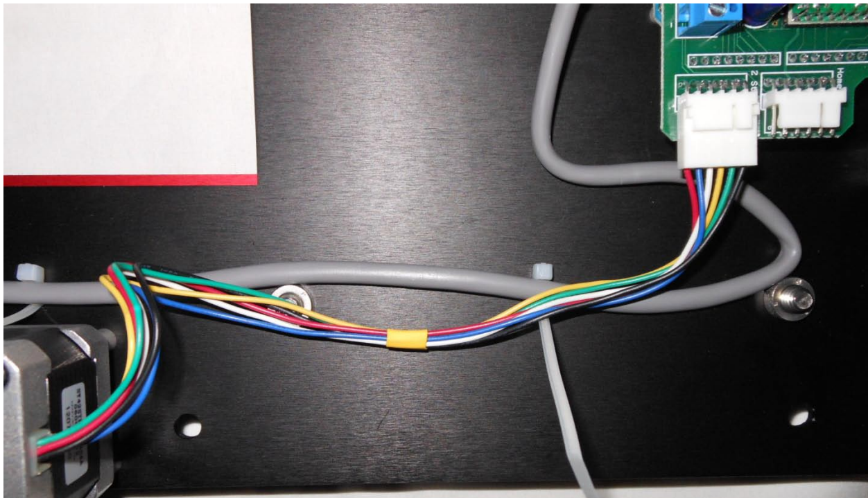
Z Axis Motor connected to Shield
