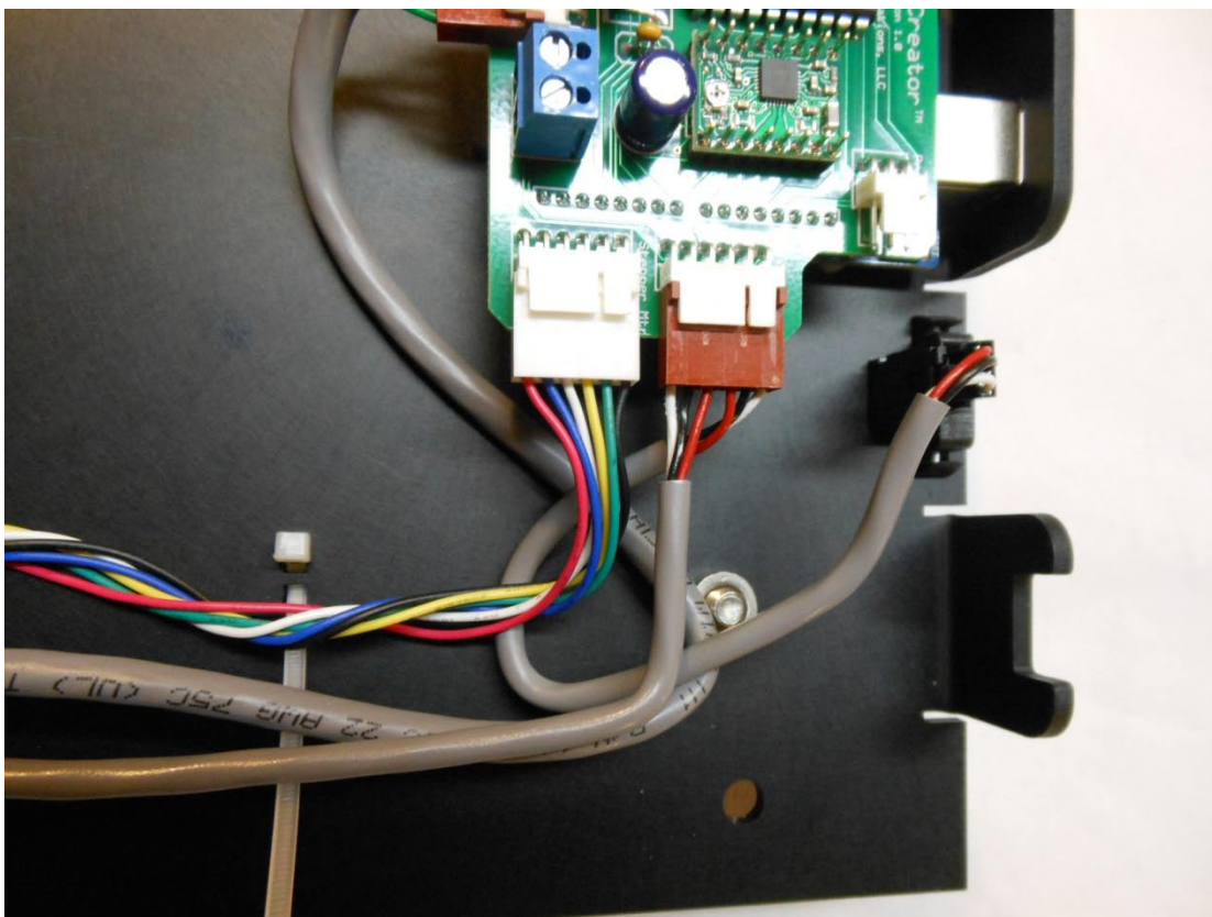
Home sensor harness connected to Shield, short run connected to Vat Table Home Sensor.
