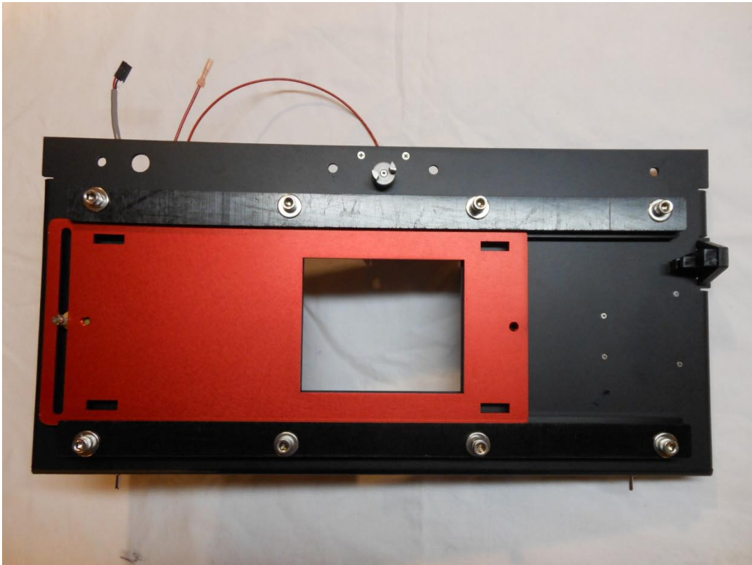
Completed XA (Horizontal Slide Base) Assembly
