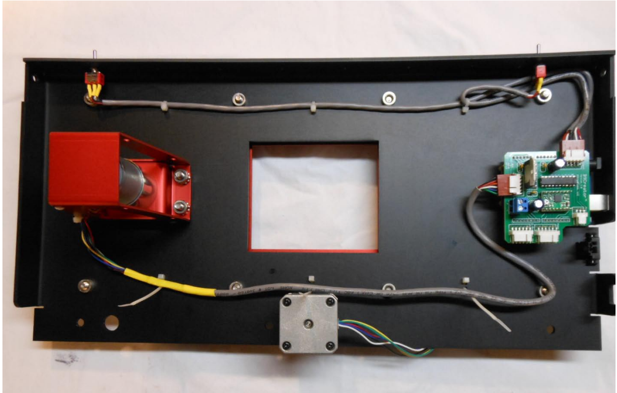
X Axis Slide Motor connected to Shield
