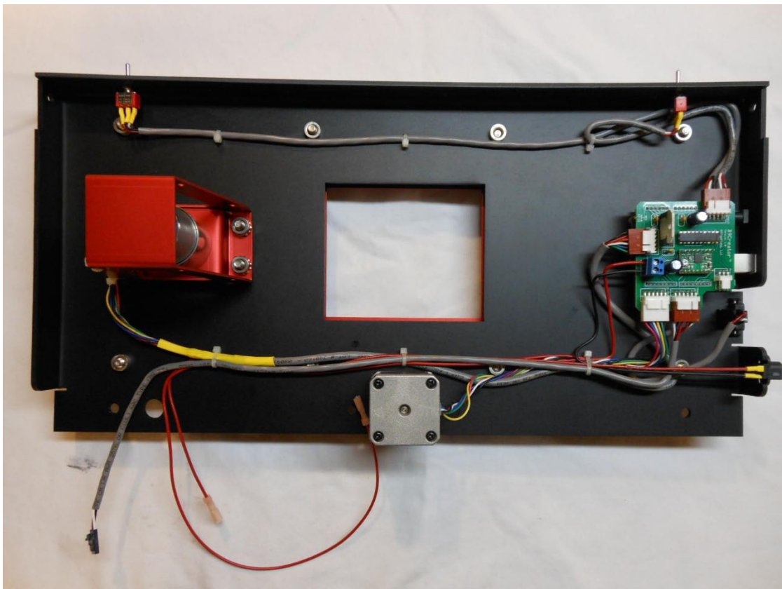
Harnesses secured and excess zip tie ends clipped off.
