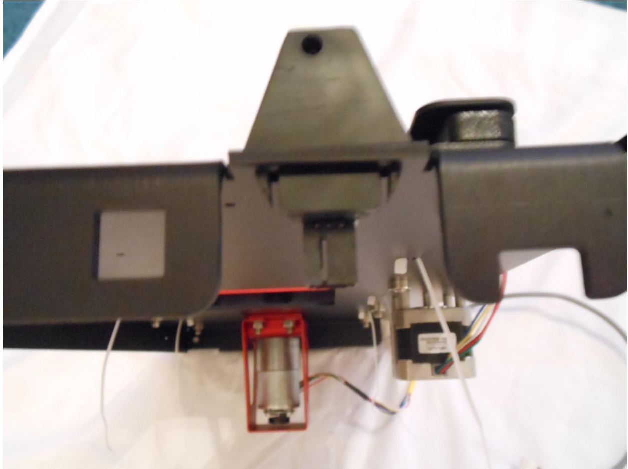
Vat Table Home Sensor snapped into place.
