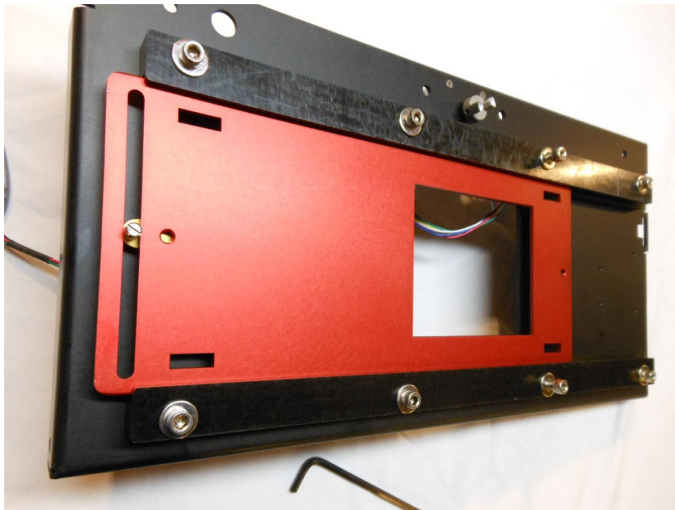
Front track in place, ready to tighten screws. Use a hex wrench to gently tighten the four screws on the "slot" side and the two on opposite side, do not overtighten. Only hand tighten the other two screws as they will be removed later when we attach the sweeper assembly.
