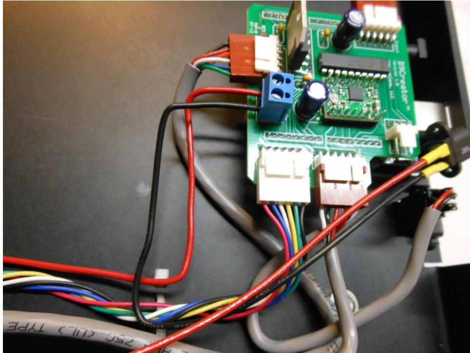
Power cable 2 in place with bare end connected to positive (+) Shield terminal
